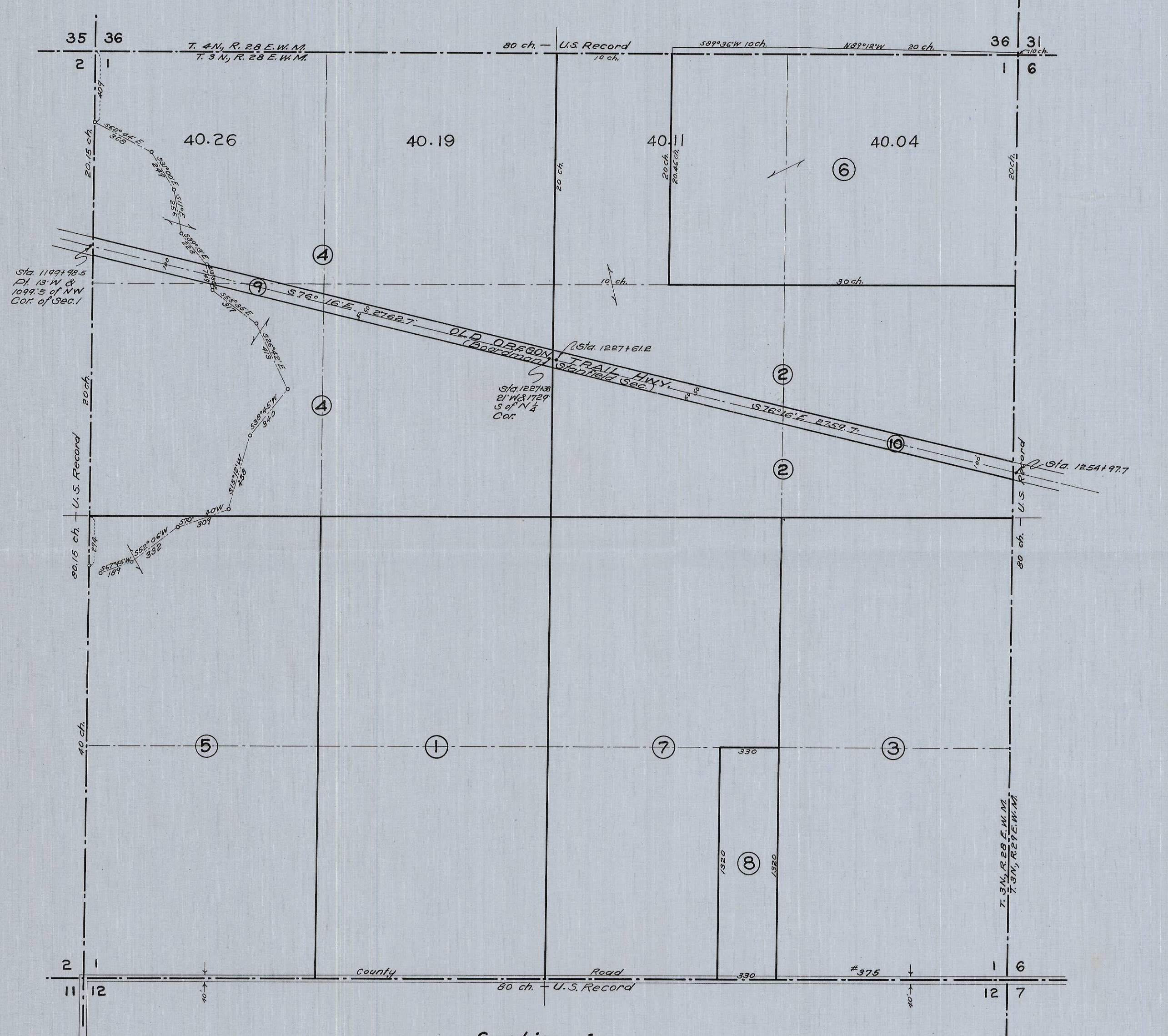
Section 1 T.3N., R.28E.W.M. Scale 1 inch = 500 feet.
