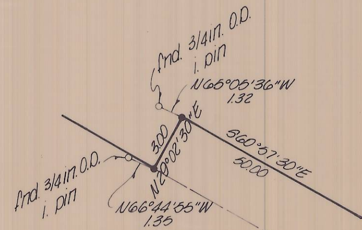
DETAIL "A" 1" = 5'
