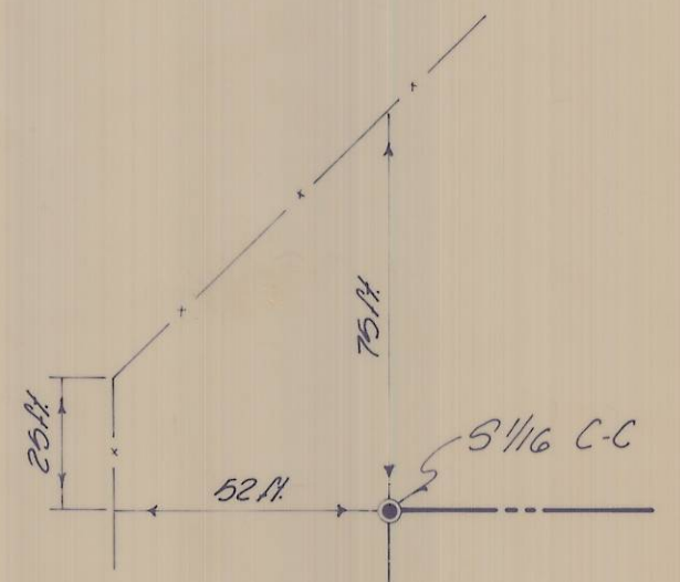
FENCE DETAIL "B" n.s.
